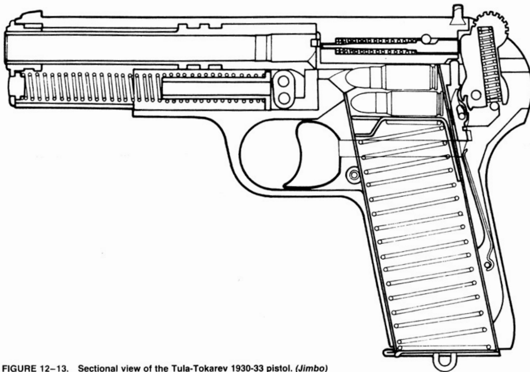
FIGURE 12-13. Sectional view of the Tula-Tokarev 1930-33 pistol. (Jimbo)
